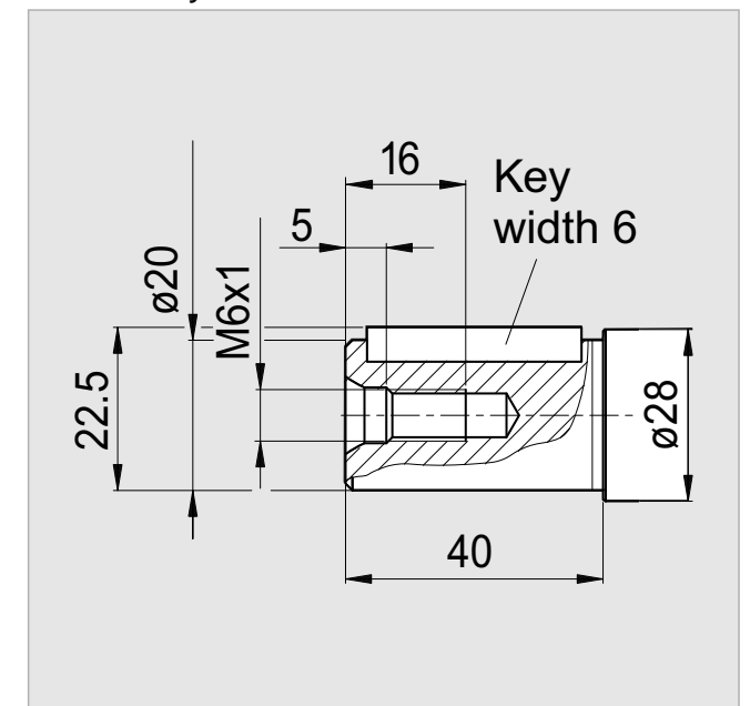
Parallel Keyed Shaft: DIN 6885 6x6x32
