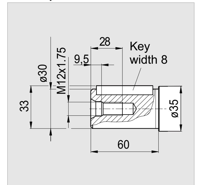
Parallel Keyed Shaft: DIN 6885 8x7x50
