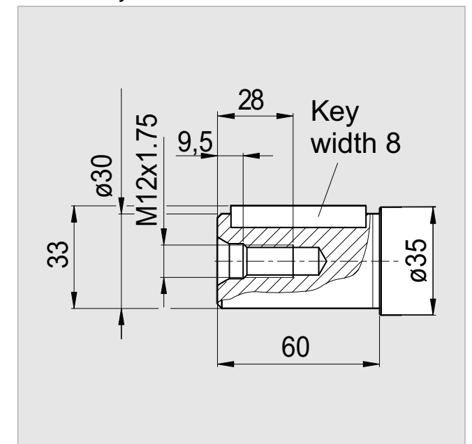
Parallel Keyed Shaft: DIN 6885 8x7x50
