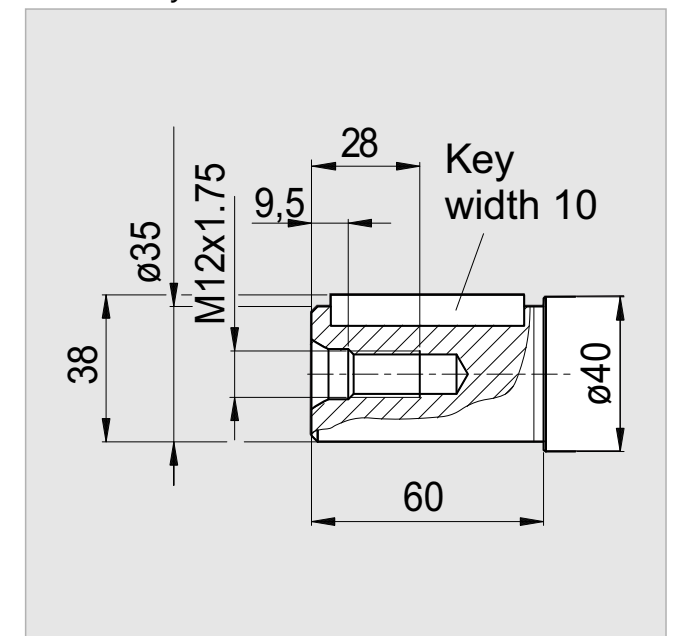
Parallel Keyed Shaft: DIN 6885 10x8x50
